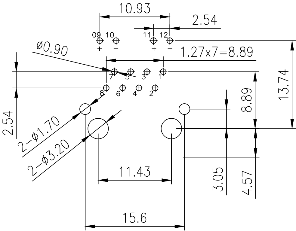
PCB Layout
